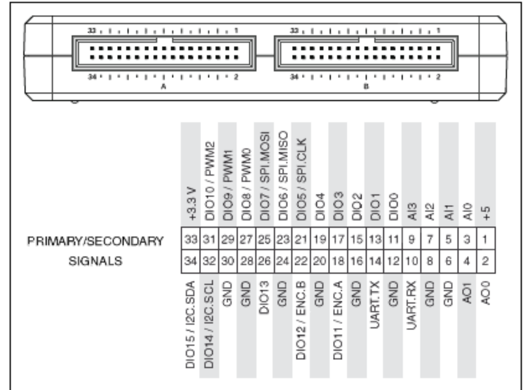
myRIO Extension Ports (MXP) Connectors
